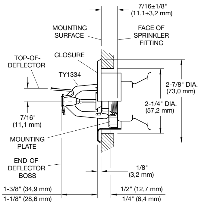
FIGURE 2 STYLE 20 RECESSED ESCUTCHEON FOR USE WITH THE SERIES LFII RESIDENTIAL HORIZONTAL SIDEWALL SPRINKLER (TY1334)
