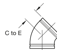
FIGURE 501 CAST 45° ELBOW
